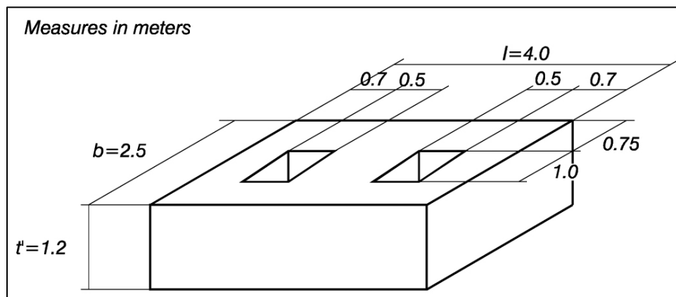
Figure VI-5-52. Example of Japanese foot protection block
