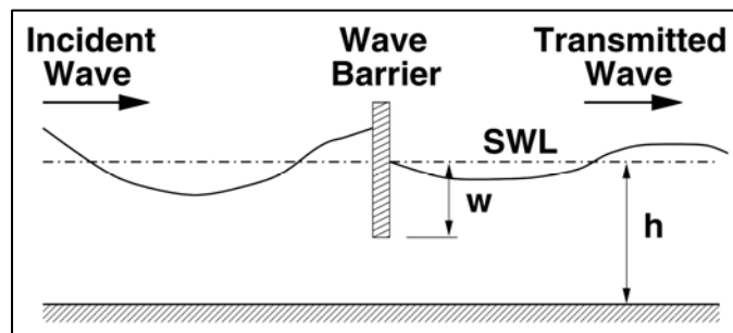
Figure VI-5-61. Wave barrier definition sketch
